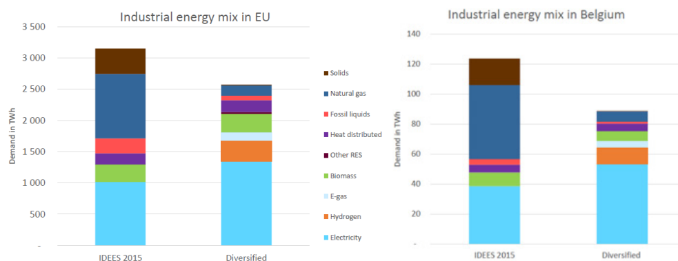
Graph 17 Industrial energy mix in the EU (left) and in Belgium (right), Diversified Energy Supply, year 2050 TWh
