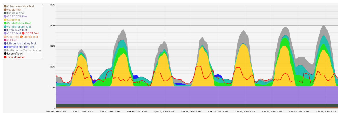
Graph 12 Graphical illustration of power generation, Diversified Energy Supply, Test Case 0, Belgium, April 16-23, 2050
