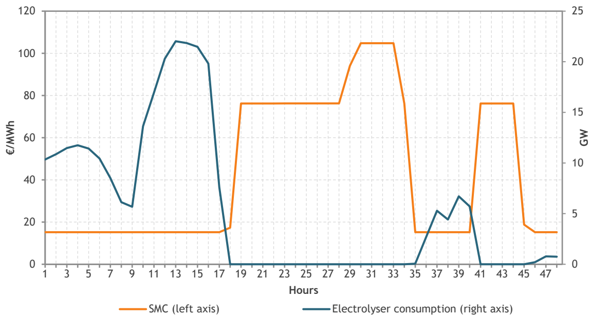
Graph 13 Illustration of power consumption of the electrolyzers versus the system marginal costs (SMC), Diversified Energy Supply, Test Case 0, February 16-18, 2050
